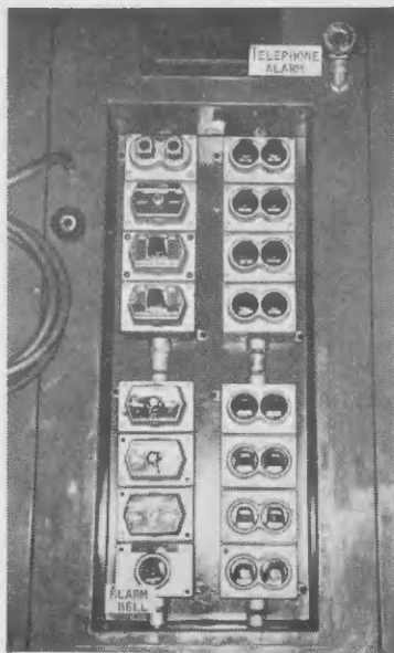
Panel inside elevator cage, with double row of push buttons at right for 14 floors. The two lower buttons at right are to open and close doors.
